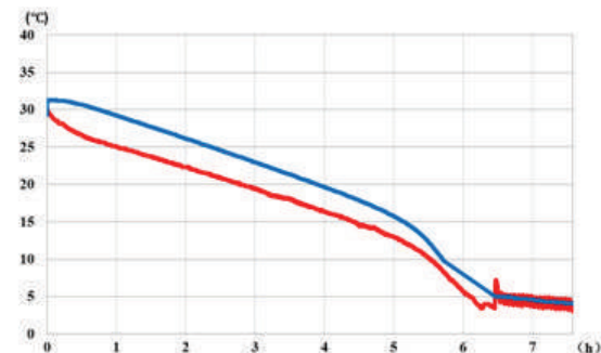
Variation of the water temperature in the container, while the ambient temperature is -35^\circ\text{C} , with a surface load of 0.1 \text{ W}/\text{cm}^2 (300W). It can be seen that despite the increased heating power, the internal temperature of the tank continues to fall slowly
